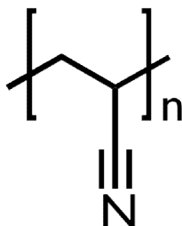
Acrylonitrile copolymer
